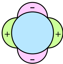
d-wave High- T_c cuprates
