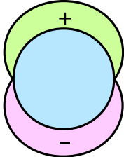
p-wave ( p_y )
